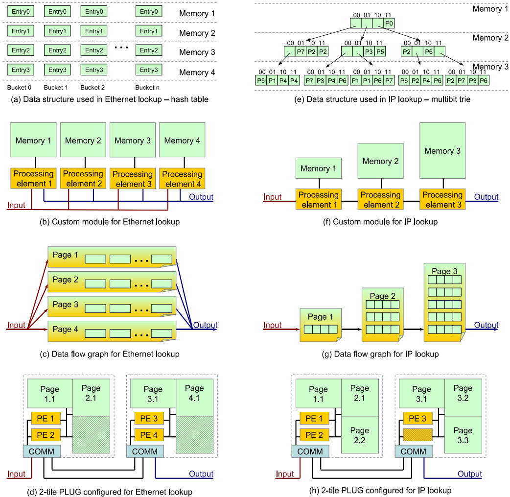
Figure 1: Data structures used by the forwarding tables for Ethernet and IP, separate custom lookup modules for them, data flow graphs describing both algorithms and the mapping of both of them to the same 2-tile PLUG.
