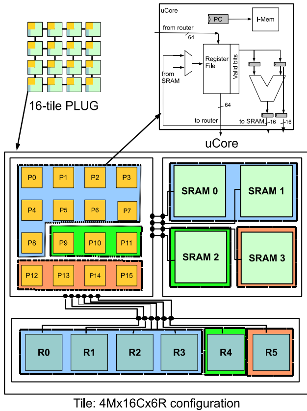
Figure 7: PLUG architecture overview showing three virtual tiles to map three logical pages.
