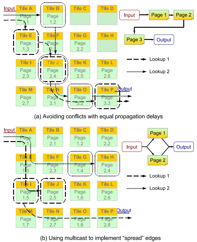
Figure 8: Mapping lookup objects to the PLUG grid.
