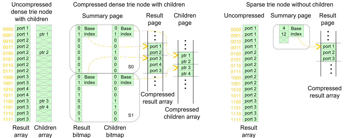
Figure 6: Compression technique and data flow graph for the IPv4 lookup object.
