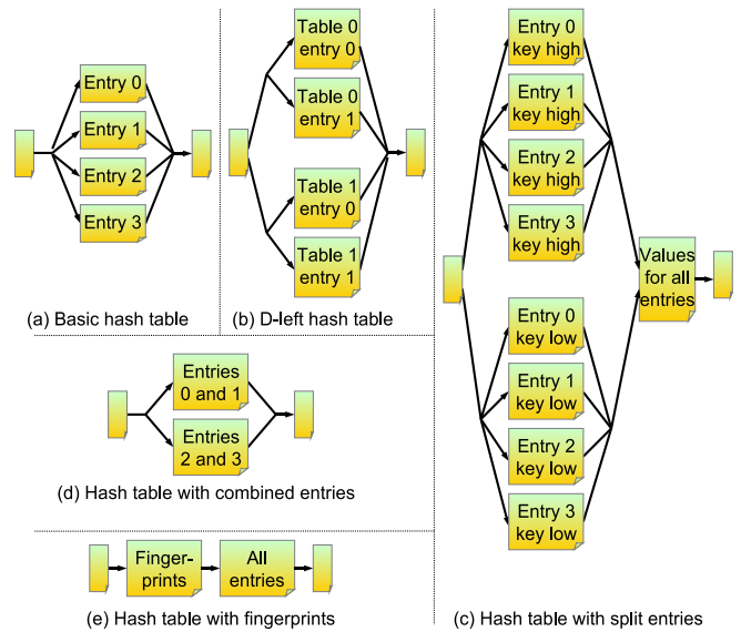
Figure 3: Data flow graphs corresponding to changes to the basic hash table design.
