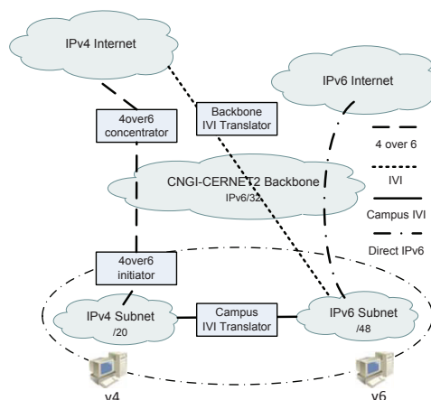
Figure 3: The Coexistence and Communication of IPv6 Users with IPv4 Users
