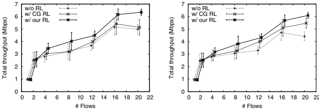
(a) RTS/CTS=OFF (b) RTS/CTS=ON
