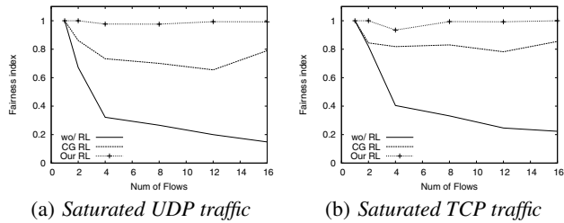
Figure 14: Fairness comparison in testbed. RTS/CTS=OFF.
