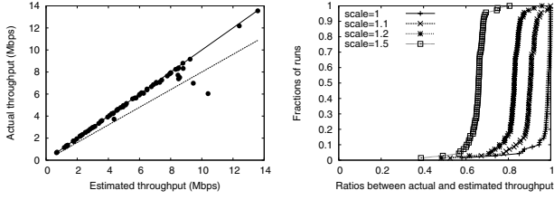
(b) Random topology, saturated UDP demands, without RTS/CTS
