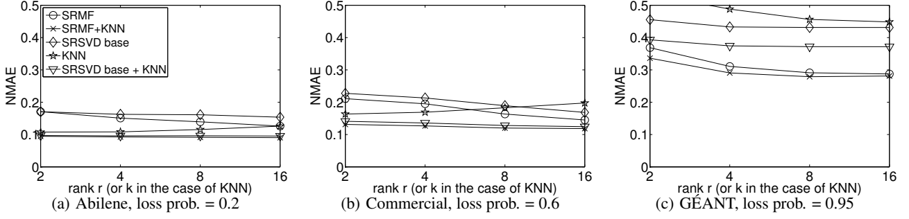
Figure 2: Sensitivity with respect to the input rank r (or k in the case of KNN).
