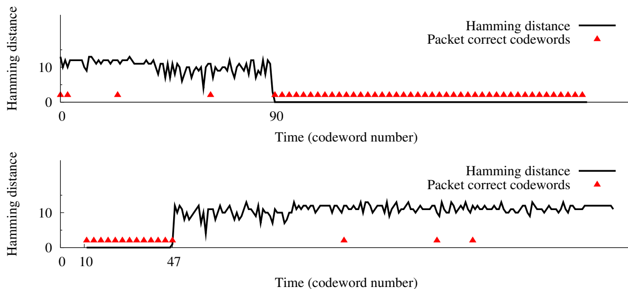
Figure 4: Partial packet reception at two different codeword synchronization offsets during a loss in codeword/symbol synchronization: codeword correctness (triangle indicators) and each codeword’s associated Hamming distance (curves). Despite uncertainty in PHY codeword timing recovery, Hamming distance indicates the correct parts of the packet to higher layers.
