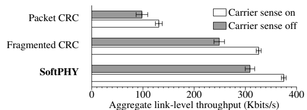
Figure 9: The impact of carrier sense on aggregate link-level throughput. Carrier sense improves throughput under each scheme, but PPR techniques yield further improvements. Postamble decoding is off in this experiment.
