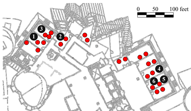
Figure 8: Experimental Zigbee testbed layout: there are 31 nodes in total, spread over 11 rooms in an indoor office environment. Each unnumbered dot indicates a Zigbee node. Software radio nodes are shown dark, labeled with numbers.
