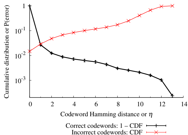
Figure 5: Distributions of Hamming distances for every codeword in every received packet, separated by whether the received codeword was correctly or incorrectly decoded. Under the threshold rule, these CDFs can be reinterpreted as curves plotting probability of misclassification.
