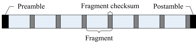
Figure 10: The per-fragment checksum approach: the packet includes multiple checksums, with each checksum taken over a different fragment of the packet.
