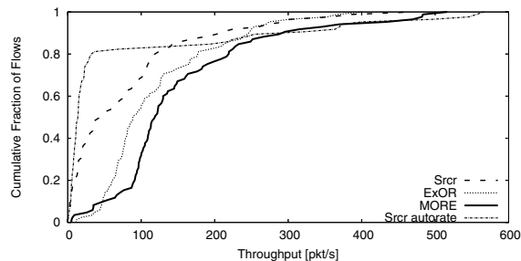
Figure 13: Opportunistic Routing Against Srcr with Autorate. The figure compares the throughput of MORE and ExOR running at 11Mb/s against that of Srcr with autorate. MORE and ExOR preserve their throughput gains over Srcr.
