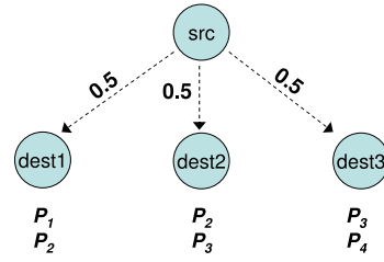
Figure 2: Multicast Example. Instead of retransmitting all four packets, the source can transmit two linear combinations, e.g., p_1 + p_2 + p_3 + p_4 and p_1 + 2p_2 + 3p_3 + 4p_4 . These two coded packets allow all three destinations to retrieve the four original packets, saving the source 2 transmissions.
