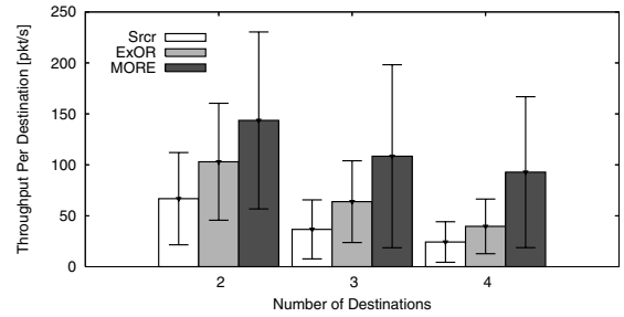
Figure 10: Multicast Throughput as a Function of the Number of Destinations for the Topology in Fig. 9. The figure shows the per-destination multicast throughput of MORE, ExOR, and Srcr. The thick bars show the average per-destination throughput taken over 40 runs with different nodes. The lines show the standard deviation.
