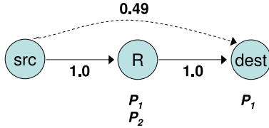
Figure 1: Unicast Example. The source sends 2 packets. The destination overhears p_1 , while R receives both. R needs to forward just one packet but, without node-coordination, it may forward p_1 , which is already known to the destination. With network coding, however, R does not need to know which packet the destination misses. R just sends the sum of the 2 packets p_1 + p_2 . This coded packet allows the destination to retrieve the packet it misses independently of its identity. Once the destination receives the whole transfer ( p_1 and p_2 ), it acks the transfer causing R to stop transmitting.
