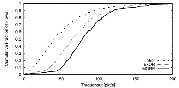
Figure 6: Unicast Throughput. Figure shows the CDF of the unicast throughput achieved with MORE, ExOR, and Srcr. MORE's median throughput is 22% higher than ExOR. In comparison to Srcr, MORE achieves a median throughput gain of 95%, while some source-destination pairs show as much as 10-12x.
