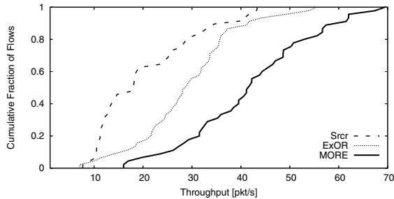
Figure 8: Spatial Reuse. The figure shows CDFs of unicast throughput achieved by MORE, ExOR, and Srcr for flows that traverse 4 hops, where the last hop can transmit concurrently with the first hop. MORE’s median throughput is 45% higher than ExOR.
