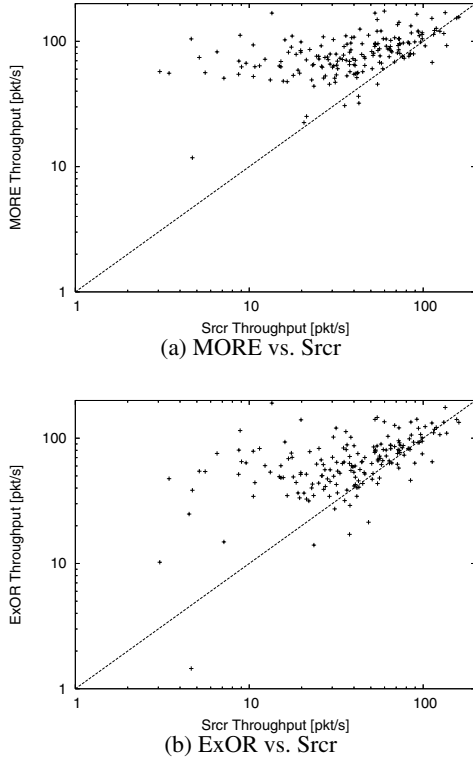
Figure 7: Scatter Plot of Unicast Throughput. Each point represents the throughput of a particular source destination pair. Points above the 45-degree line indicate improvement with opportunistic routing. The figure shows that opportunistic routing is particularly beneficial to challenged flows.
