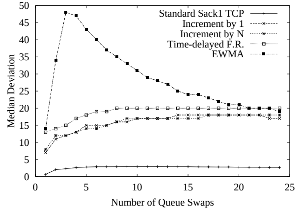
Figure 8: Median deviation of unnecessary retransmissions.
