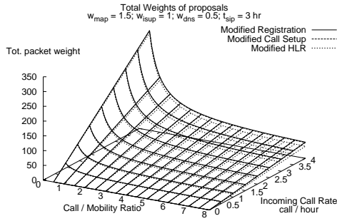
Figure 14: Weighted signalling load of the three proposals: non-IP-enabled visited network
