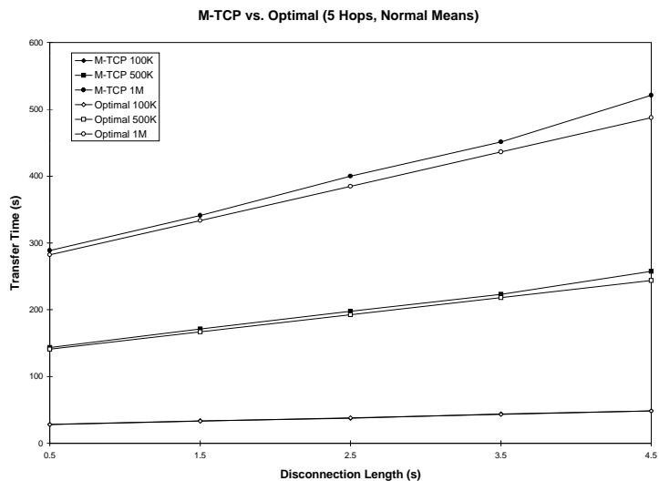
Figure 9: M-TCP vs. Optimal performance.
