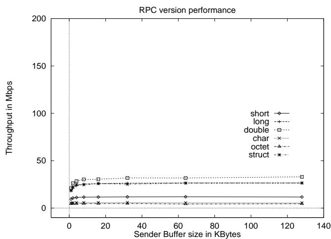
Figure 12: Performance of the RPC Loopback Version of TTCP
