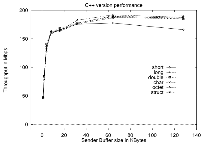
Figure 11: Performance of the C++ Wrappers Loopback Version of TTCP
