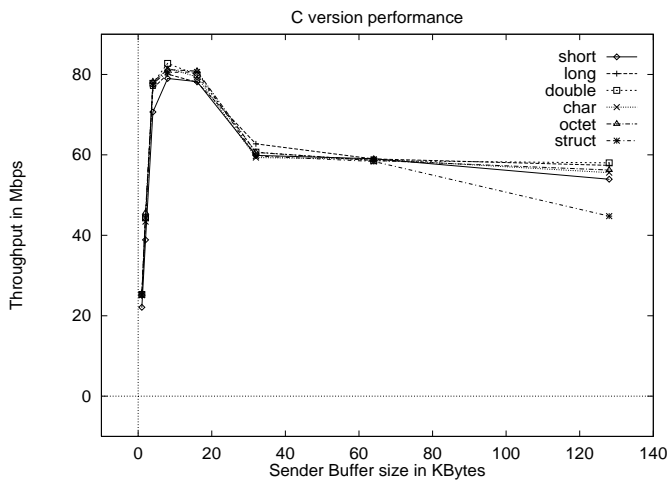
Figure 4: Performance of the Modified C Version of TTCP
