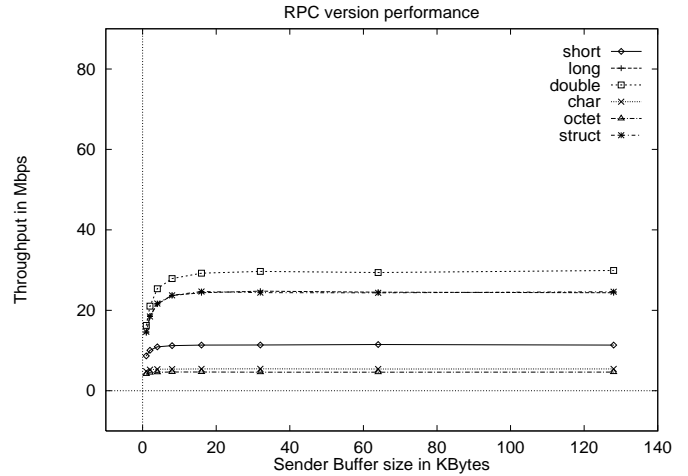
Figure 6: Performance of the RPC Version of TTCP
