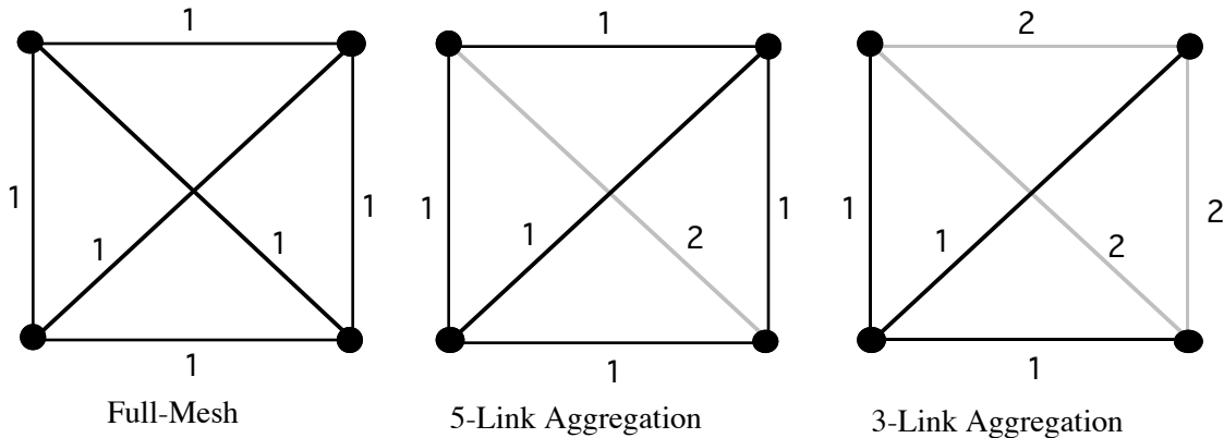
Figure 4: Aggregation of a Topology with a Constant Metric Weight
